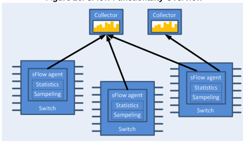
Figure 26: sFlow Functionality Overview
