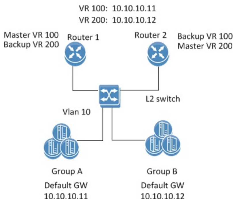
Figure 34: Common VRRP Configuration with Load Balancing
