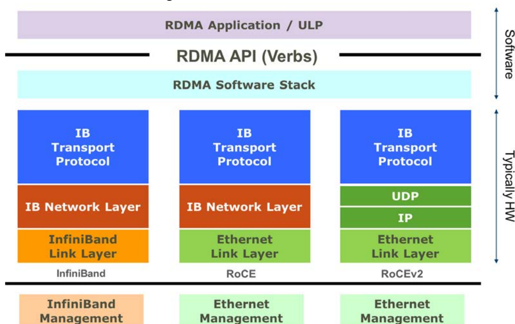
Figure 28: RoCEv2 Protocol Stack
