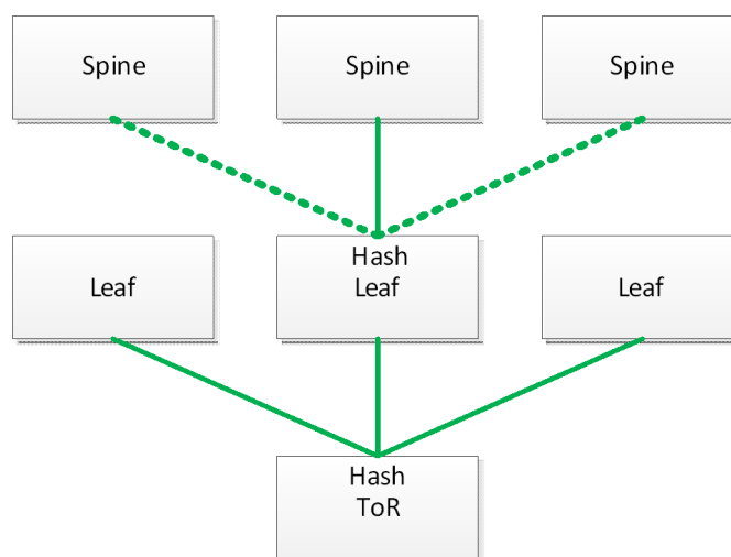
Figure 31: Multiple Hash Functions
