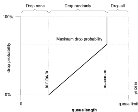
Figure 21: RED/ECN Drop Profiles
