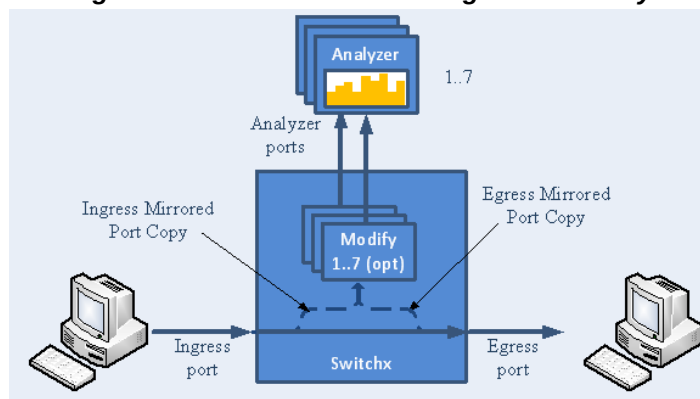
Figure 22: Overview of Mirroring Functionality
