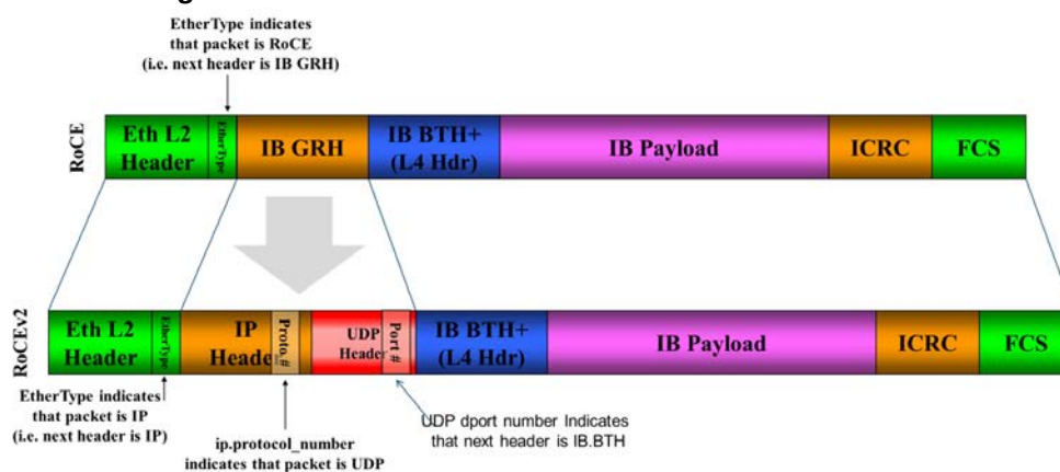
Figure 27: RoCEv2 and RoCE Frame Format Differences
