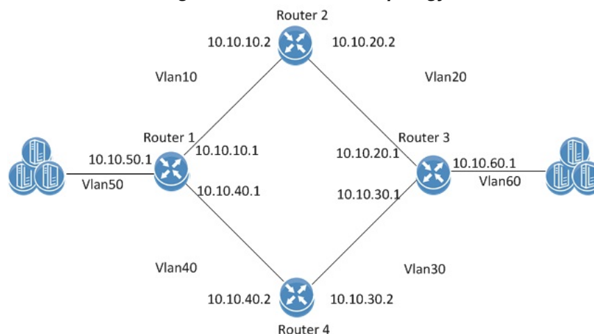
Figure 32: OSPF Basic Topology
