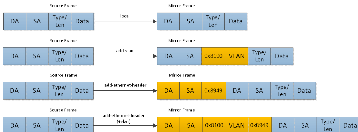
Figure 24: Header Format Options
