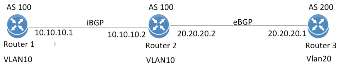
Figure 33: Basic BGP Configuration
